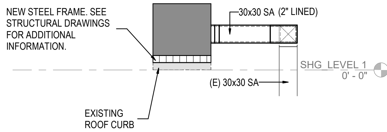
1 AC SECTION VIEW - NORTH SOUTH SCALE: 1/8" = 1'-0"
