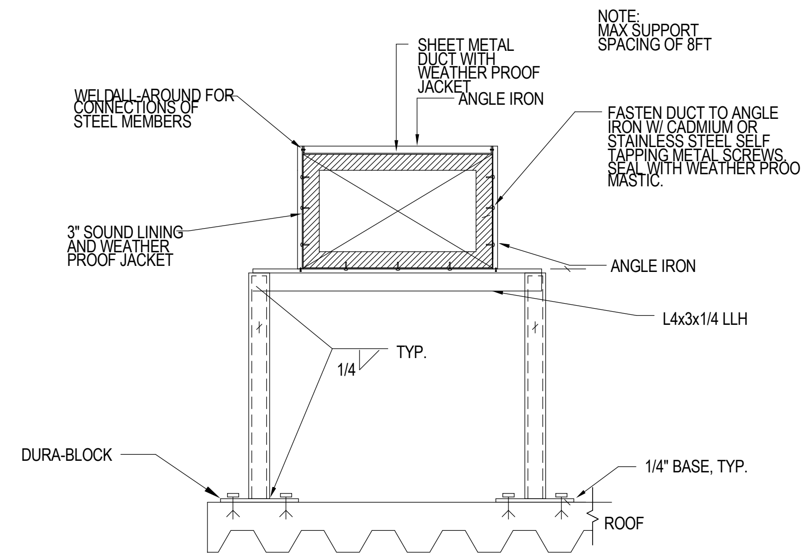
2 DUCT ROOF MOUNTED SUPPORT DETAIL SCALE: NONE
