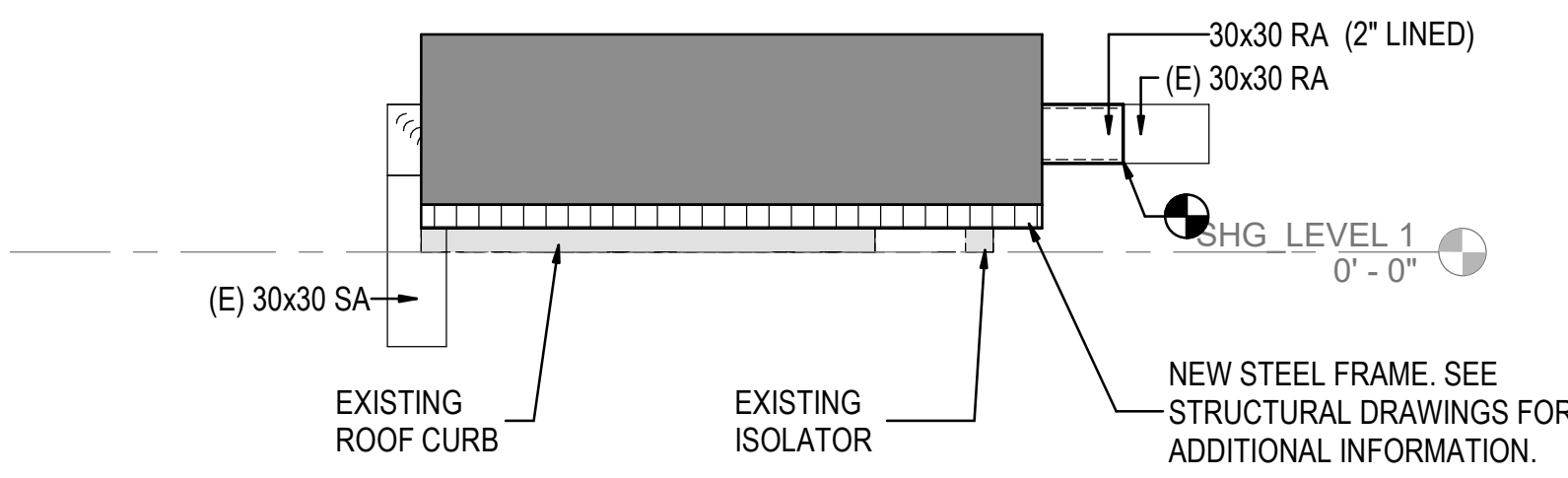
2 AC SECTION VIEW - EAST WEST SCALE: 1/8" = 1'-0"
