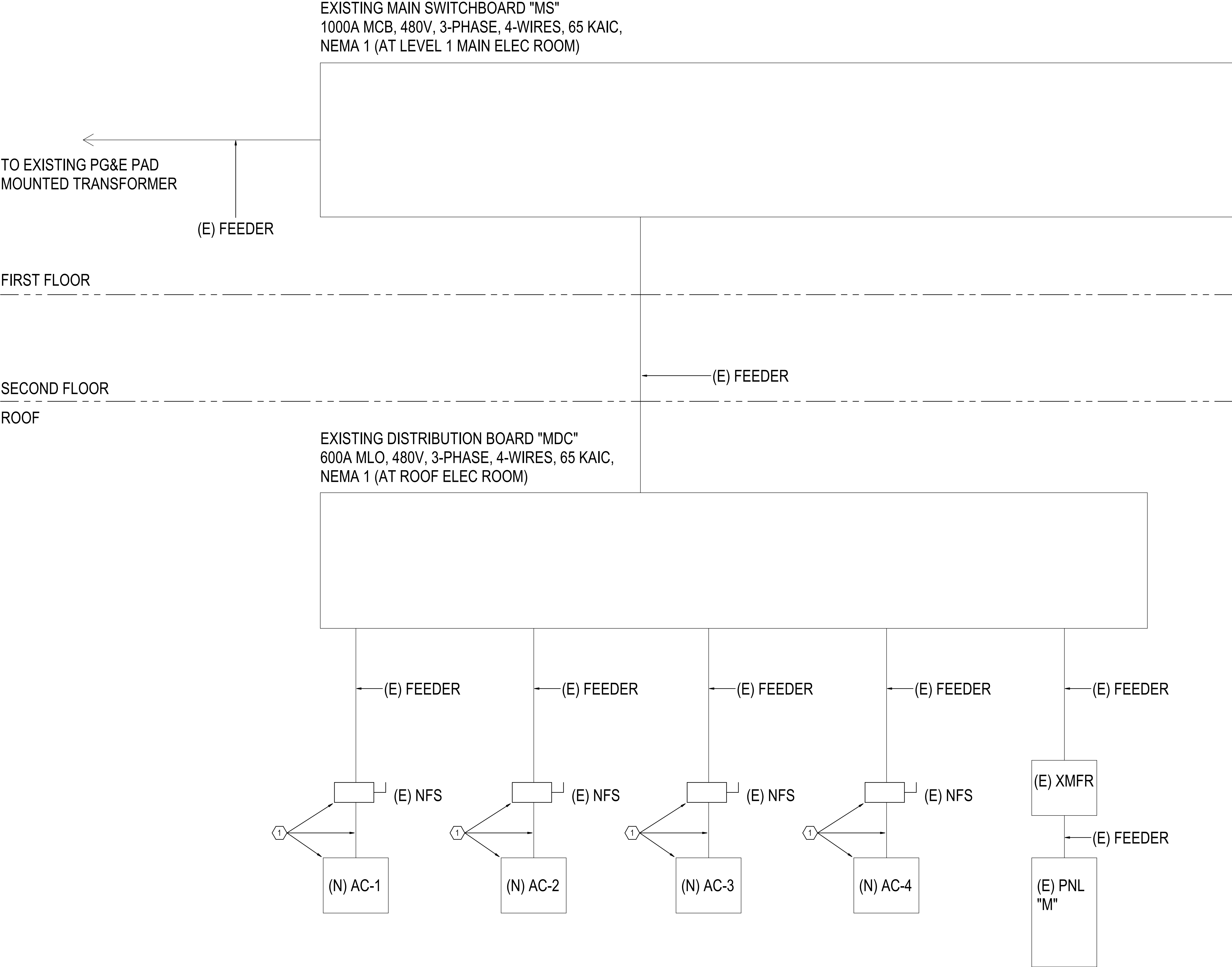
ELECTRICAL SINGLE LINE DIAGRAM
